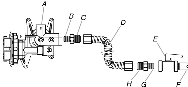
A. Gas pressure regulator B. Use pipe-joint compound. C. Adapter (must have 1/2" male pipe thread) D. Flexible connector E. Manual gas shutoff valve F. 1/2" or 3/4" gas pipe G. Use pipe-joint compound. H. Adapter
