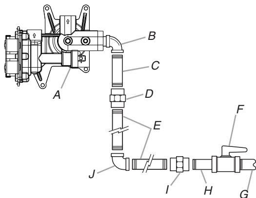
A. Gas pressure regulator B. 90° elbow (must have 1/2" male pipe thread) C. Nipple D. Union E. Black iron pipe F. Manual gas shutoff valve G. 1/2" or 3/4" gas pipe H. Nipple I. Union J. 90° elbow
